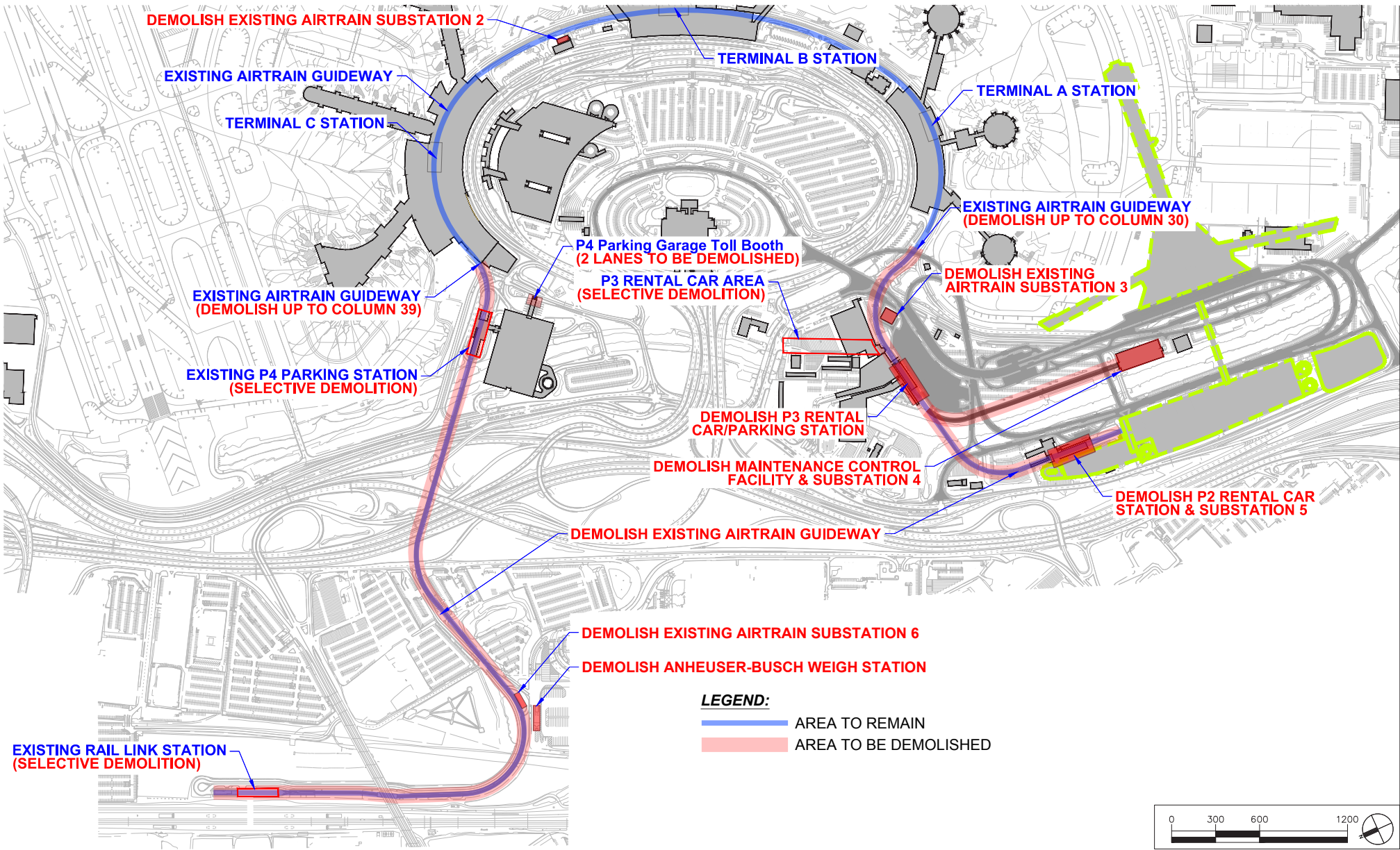
FIGURE 5: AirTrain EWR Replacement Program Demolition Plan
